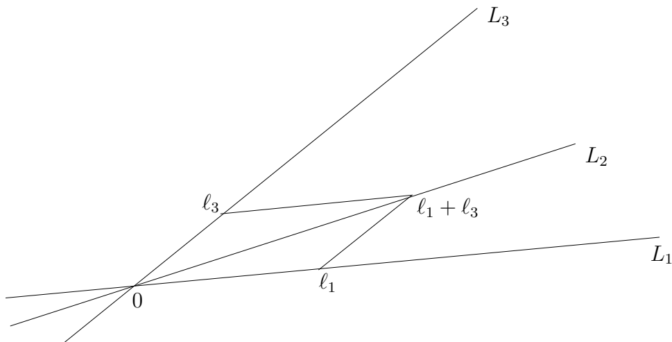
FIGURE 2. Let L_1 and L_2 be transverse to L_3 . Then the vector l_3 \in L_3 is the image of the vector l_1 \in L_1 under the isomorphism T_{13} : L_1 \rightarrow L_3 defined by L_2 . The value at l_1 of the quadratic form Q_L^{L_1, L_3} on L_1 based at L_3 and induced by L_2 measures the signed area of the parallelogram with vertices 0, l_1, l_1 + l_3, l_3 . Moreover, if also L_1 and L_2 are transverse, then Q_L^{L_1, L_3}(l_1) = -Q_L^{L_3, L_1}(l_3) , where l_1 and l_3 are related as above.
