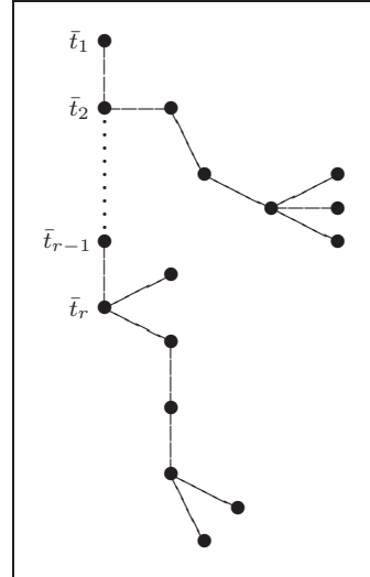
The quotient T/\langle\sigma\rangle
