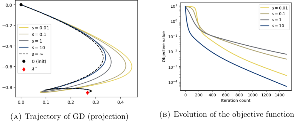
FIGURE 2.2. Behavior of the limit model and effect of the scale parameter s . (left) Projection of \lambda^m(t) on the two first coordinates. (right) Evolution of the loss.
