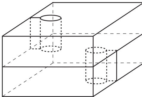
Figure 5.5. Bing's house with two rooms
