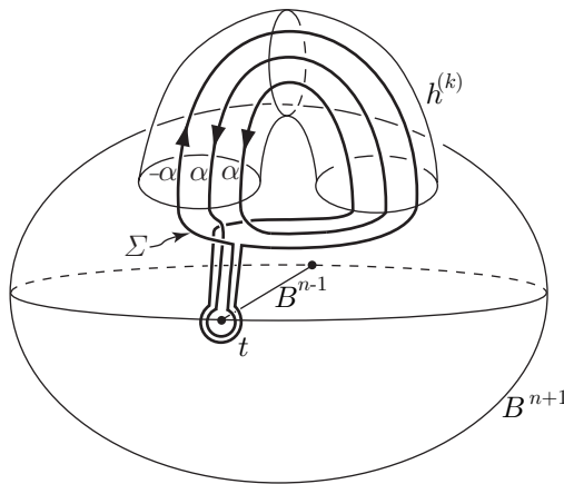
Figure 6.2. \Sigma is the attaching sphere for the (k + 1) -handle
