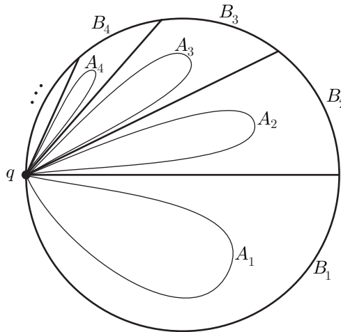
Figure 2.40. A sequence of cells whose union is a cell
