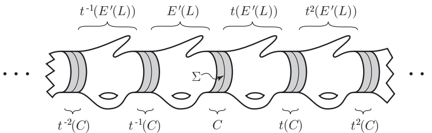
Figure 6.11. The cyclic cover \tilde{E}_k(L)
