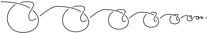
Figure 2.25. A tame arc
