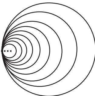
Figure 0.2. The Hawaiian earring
