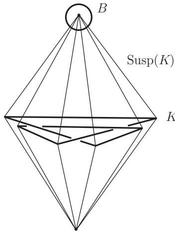
Figure 1.6. \partial B contains a small copy of K and B \cap \text{Susp}(K) is a cone
