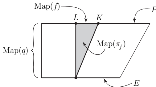
Figure 5.2. Proof of Lemma 5.1.8
