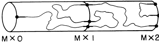
Figure 15. Pasting together two cobordisms within M
