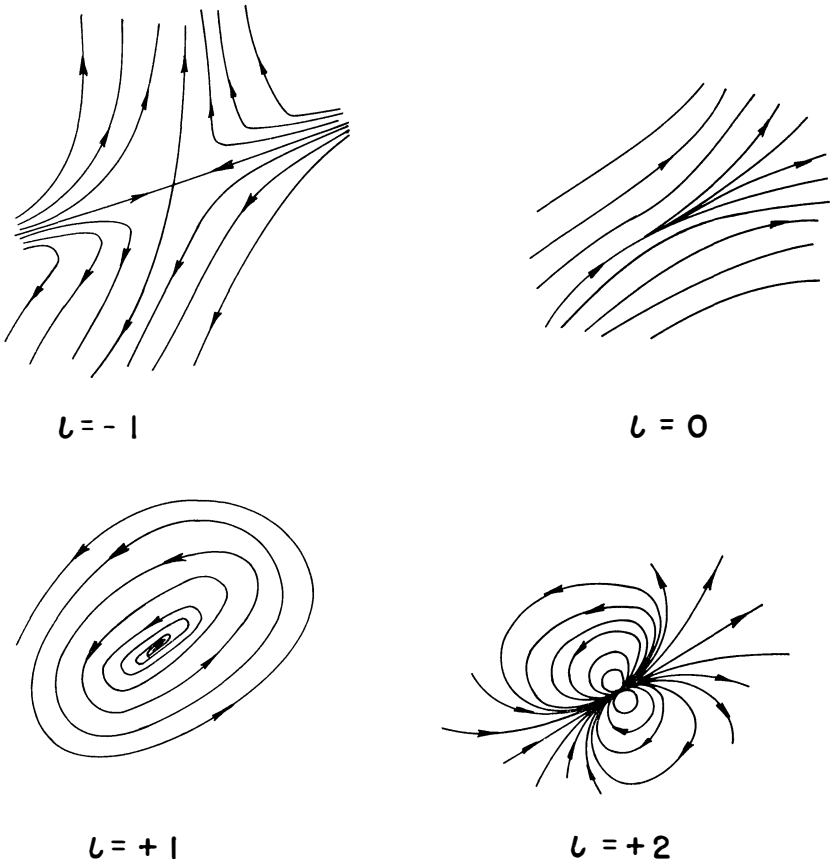
Figure 12. Examples of plane vector fields
