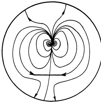
Figure 13. An example with index sum +1
