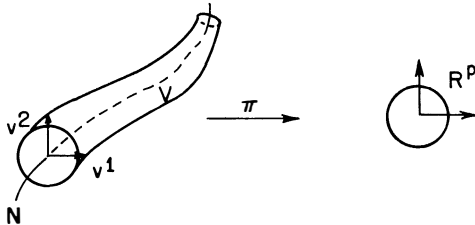
Figure 18. Constructing a map with given Pontryagin manifold
