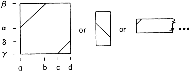
Figure 19. Three of the possibilities for \Gamma
