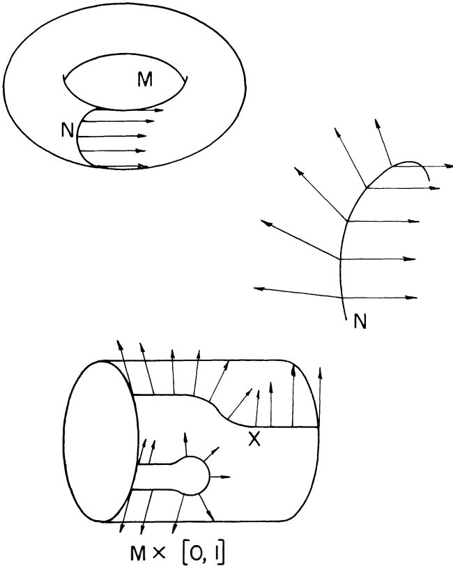
Figure 16. Framed submanifolds and a framed cobordism
