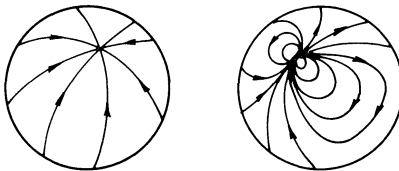
Figure 11 (below). Attempts for n = 2
