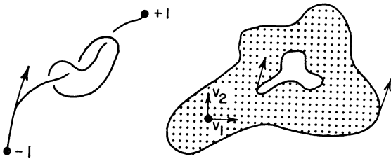
Figure 8. How to orient a boundary
