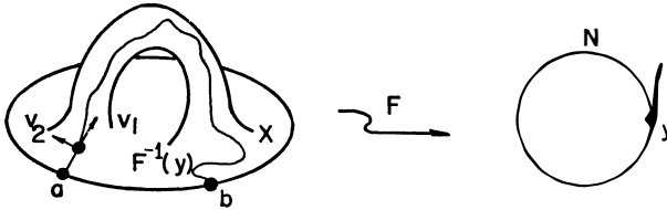
Figure 9. How to orient F^{-1}(y)
