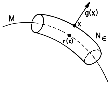
Figure 14. The \epsilon -neighborhood of M
