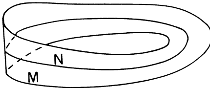
Figure 17. An unframable submanifold
