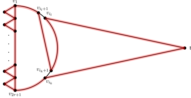
Figure 1: An illustration of how an edge between two elements v_{i_k+1}, v_{i_{k+1}} of S can be used to construct a new C_{\ell'}^r .
