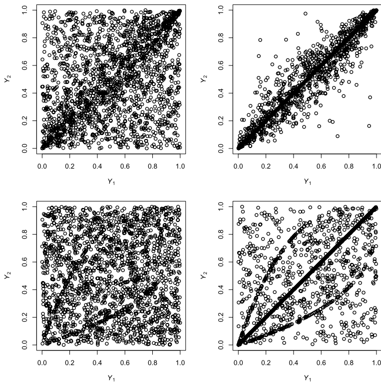
FIG. 2. Scatter plots of 2000 samples from \mathbf{Y} for \mathbf{V} \sim \Pi and \mathbf{U} following a bivariate ( m = 2 ) t_3 copula with Kendall's tau equal to 0.75 (top row) or a survival Marshall–Olkin copula with parameters \alpha_1 = 0.25, \alpha_2 = 0.75 (bottom row). For the plots on the left-hand side, the number of rows of X with one 1 are randomly chosen among \{0, 1, 2 (= d)\} , the corresponding rows and columns are then randomly selected among \{1, 2 (= d)\} and \{1, 2 (= m)\} , respectively. For the plots on the right-hand side, X is drawn from a multinomial distribution with probabilities 0.5 and 0.5 such that each row contains precisely one 1.
