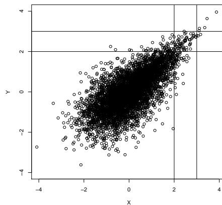
(b) Gumbel copula C_\theta^{\text{gum}} with \theta := 2 .
