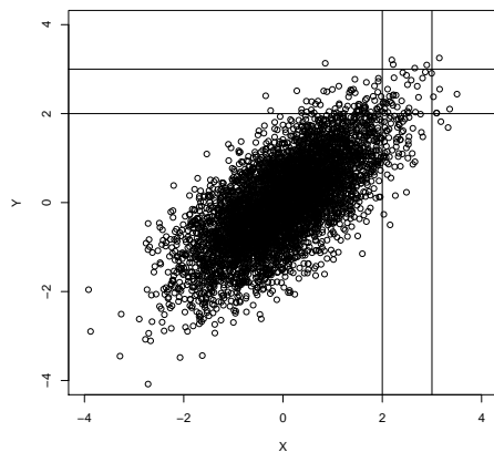
(a) Gaussian copula C_\rho^{\text{gau}} with \rho := 0.7 .
