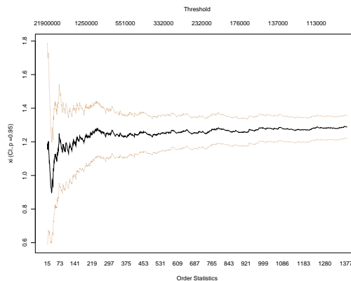
Figure 4: Hill plot for g = 4, h = 0.2 and n = 10^6 .
