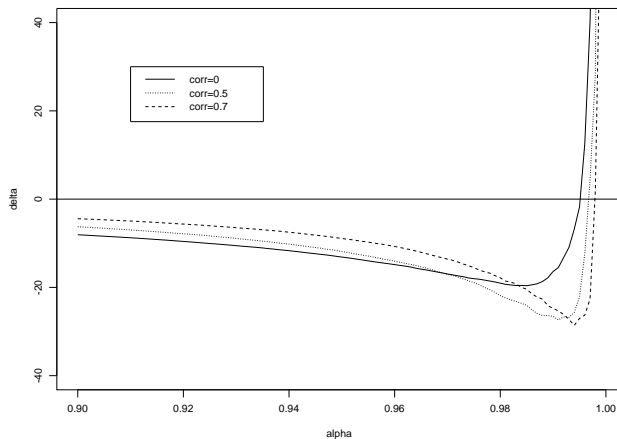
Figure 8: Plot of \delta_{g,h}(\alpha) as a function of \alpha for g = 2.4 , h = 0.2 , n = 10^7 and Gauss-copula with correlation \rho = 0, 0.5 and 0.7 . Note that \rho = 0 corresponds to the independence case in Figure 6.
