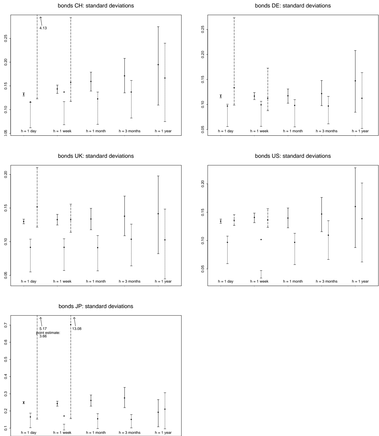
Figure 3 10-year government bonds: estimates for standard deviations (including confidence intervals constructed via simulation), using random walk models (full lines), AR(p) models (dotted lines) and GARCH(1,1) models (dashed lines).
