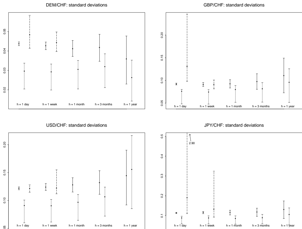
Figure 1 Foreign exchange rates: estimates for standard deviations (including confidence intervals constructed via simulation), using random walk models (full lines), AR( p ) models (dotted lines) and GARCH(1,1) models (dashed lines).
