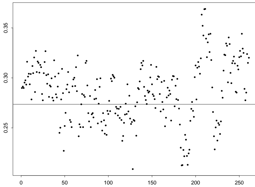
Figure 8 Point estimates for one-year 1% expected shortfall (percentage loss) for a simulated random walk, based on calibration horizons from one day to one year. Underlying model: random walk with normal innovations. The true value (horizontal line) is 27.35%.
