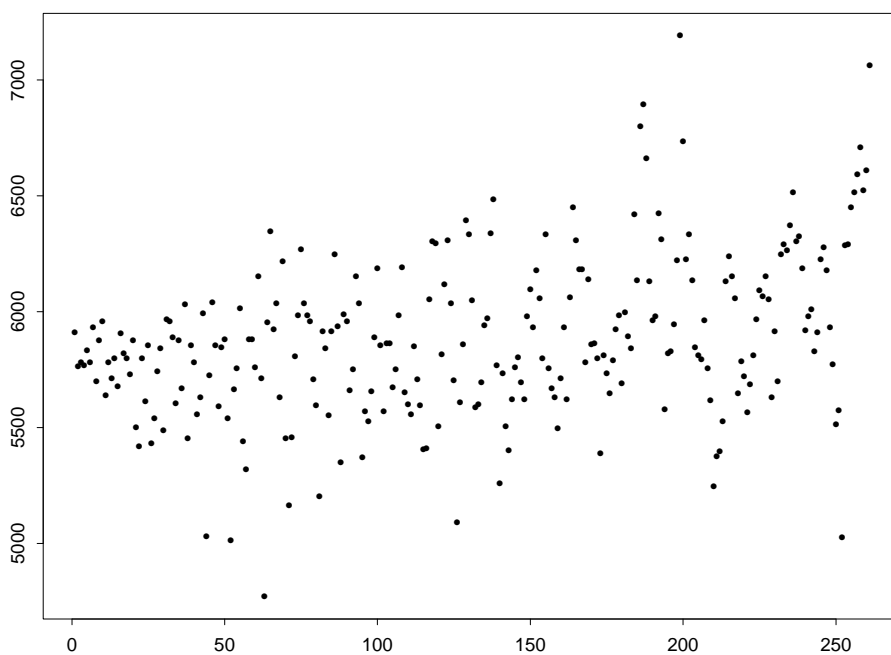
Figure 6 Point estimates for one-year 1% expected shortfall for the SMI, transformed in such a way that the values at the end of the year 2001 can be read off. The estimates are based on calibration horizons h from one day to one year. Underlying model: random walk with normal innovations.
