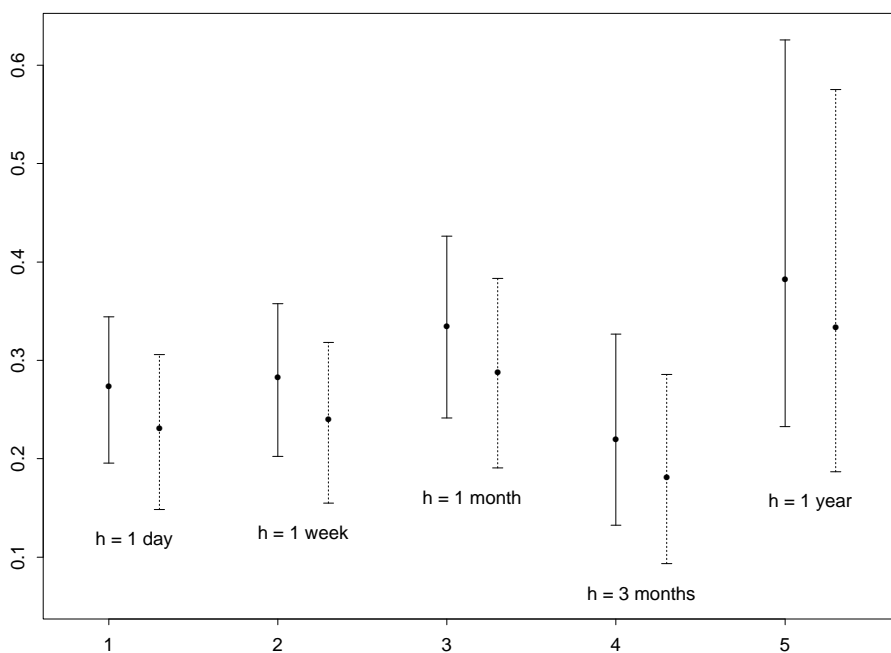
Figure 4 Point estimates and 95% confidence intervals for one-year 1% expected short-fall and 1% value-at-risk for the SMI ( percentage loss ), based on different calibration horizons h . Underlying model: random walk with normal innovations.
