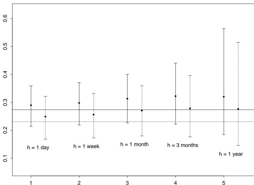
Figure 7 Point estimates and 95% confidence intervals for one-year 1% expected shortfall and 1% value-at-risk (percentage loss) for a simulated random walk, based on five different calibration horizons h . Underlying model: random walk with normal innovations. The true values (horizontal lines) are 27.35% for expected shortfall and 23.09% for value-at-risk.
