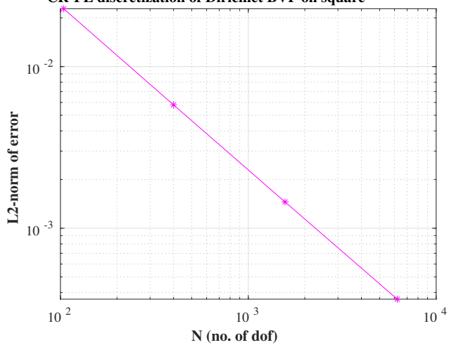
CR-FE discretization of Dirichlet BVP on square
