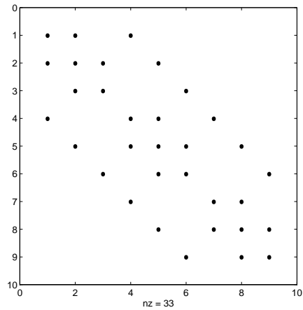
Figure 6: The sparsity pattern of a matrix
