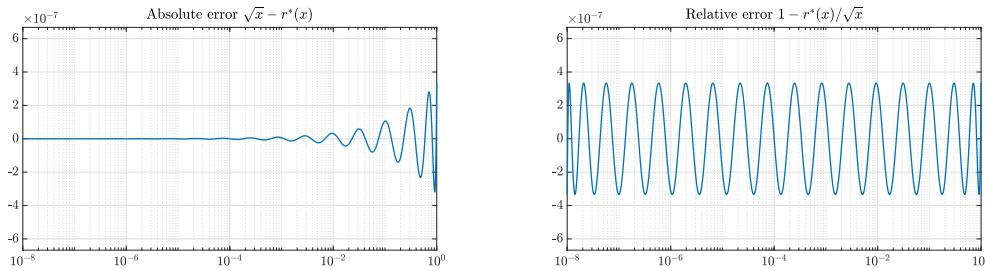
FIG. 7.3. Result of the weighted version of our barycentric Remez algorithm for the function f(x) = \sqrt{x}, x \in [10^{-8}, 1] with w(x) = 1/\sqrt{x} and a type (17, 17) rational approximation. We plot the absolute error curve on the left, while the relative error (right), matching our choice of w , gives an expected equioscillating curve. This is Zolotarev's third problem.
