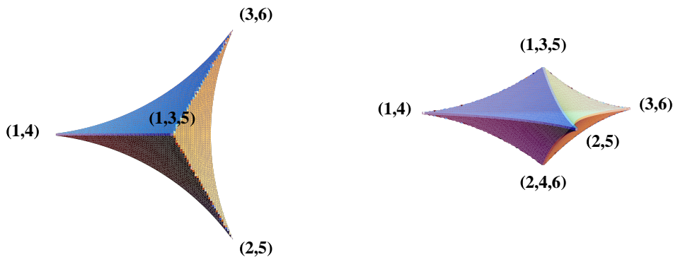
FIGURE 5. Top and side views of \overline{\mathcal{H}}_6^{eq}
