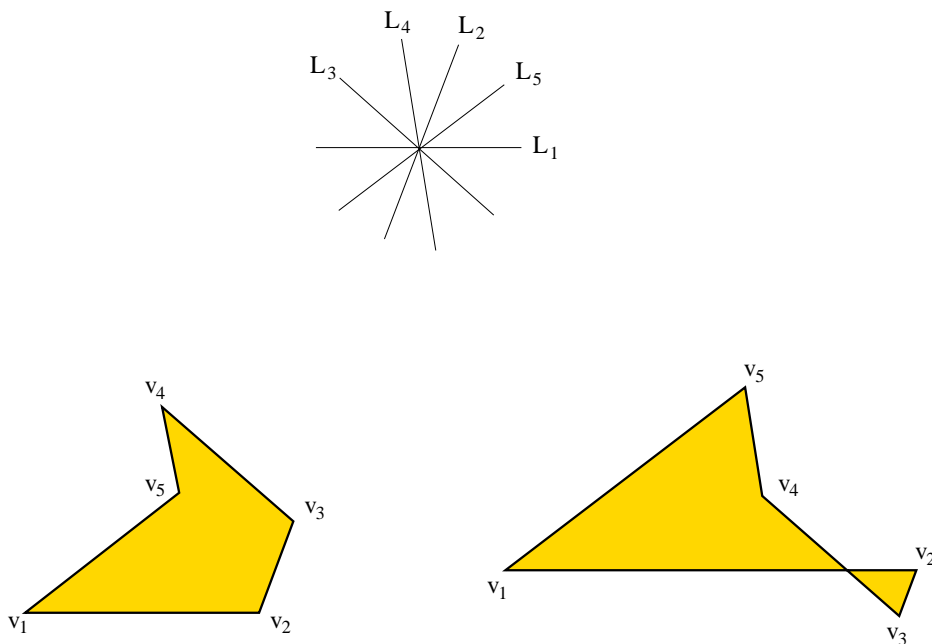
FIGURE 2. An example of a choice of lines \mathcal{L} together with two polygons in the corresponding P_n^{\mathcal{L}}
