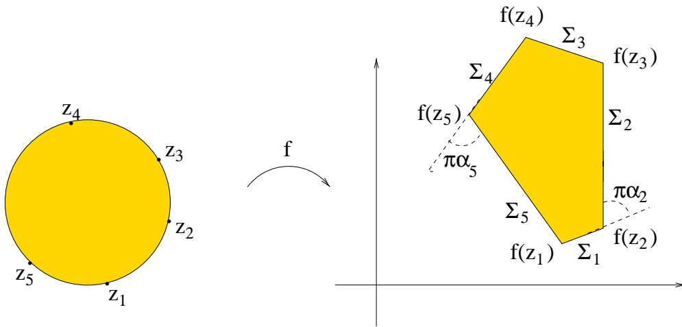
FIGURE 1. The Schwarz-Christoffel transformation
