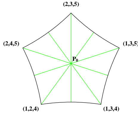
FIGURE 4. \overline{\mathcal{H}}_5^{eq} with fundamental domains for the \mathbb{D}_5 -action
