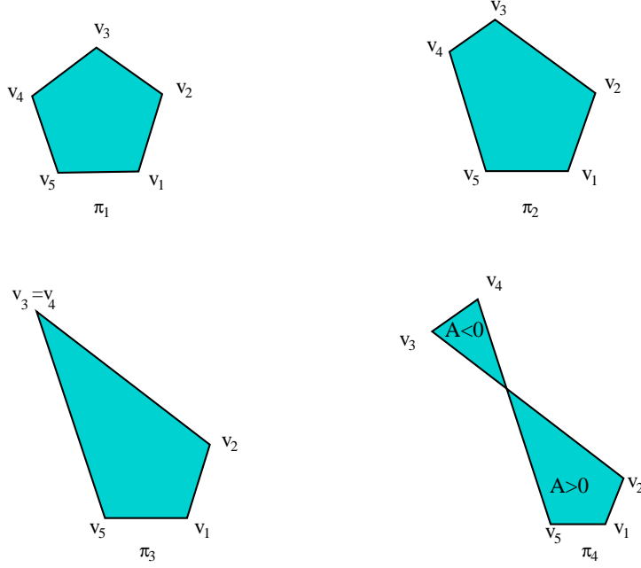
FIGURE 3. Polygons in P_n^{\mathcal{L}} : two in \mathcal{C}_n^{\mathbb{L}} , one on the boundary of \overline{\mathcal{C}}_n^{\mathbb{L}} and one outside \overline{\mathcal{C}}_n^{\mathbb{L}} but in the positive cone of A
