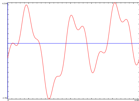
FIGURE 6.4. A trigonometric polynomial
