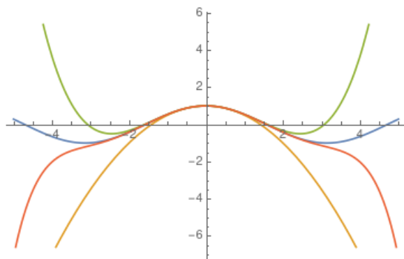
FIGURE 5.8. Taylor polynomials of cosine
