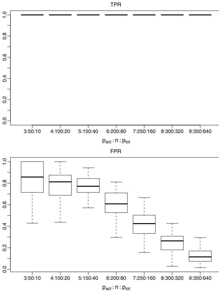
Fig. 6 Simulation 2 compares the performance of the FMRLasso for a series of models which gets “sparser” as the sample size grows. (Top) True Positive Rate (TPR); (Bottom) False Positive Rate (FPR) over 100 simulation runs
