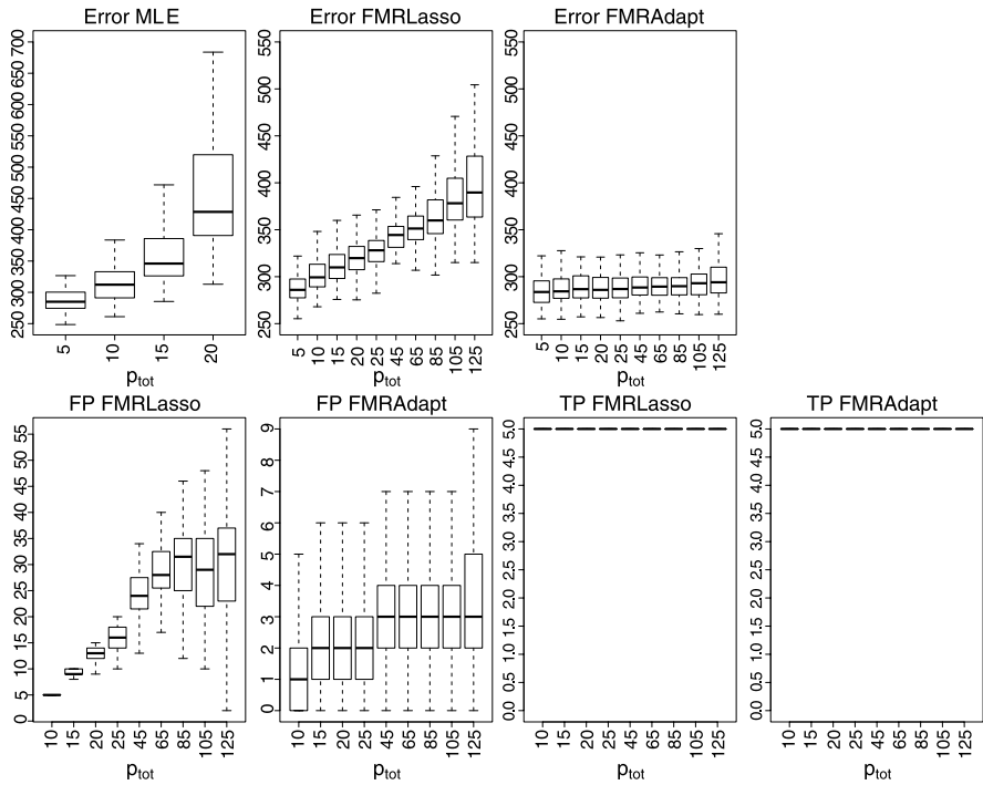
Fig. 1 Simulation 1, Model M1. (Top) Predictive log-likelihood loss (Error) for MLE, FMRLasso, FMRAdept; (Bottom) False Positives (FP) and True Positives (TP) for FMRLasso and FMRAdept
