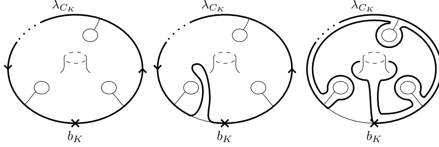
FIGURE 11. Homotopy from the path \lambda_{C_K} to \gamma_{K,m_i} * \cdots * \gamma_{K,1} * \delta_K .
