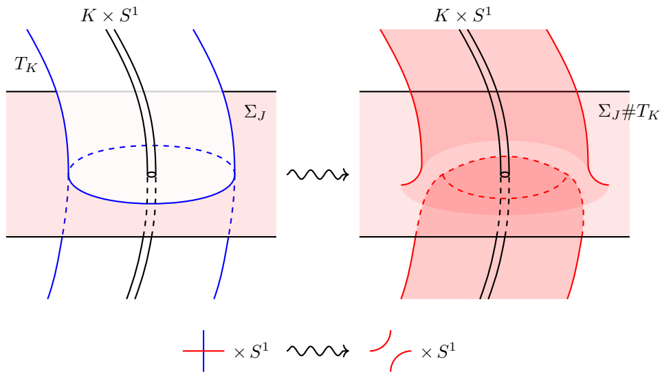
FIGURE 6. Resolving an intersection of T_K and \Sigma_J to create a connected surface.
