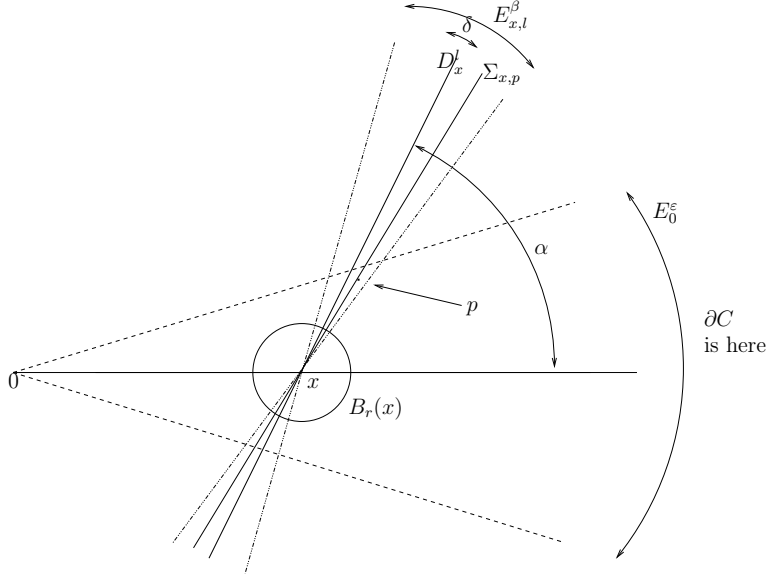
Figure 4: The objects involved: with C , as in the proof, we mean C_{x_0, \rho_n} \lrcorner B_1 .
