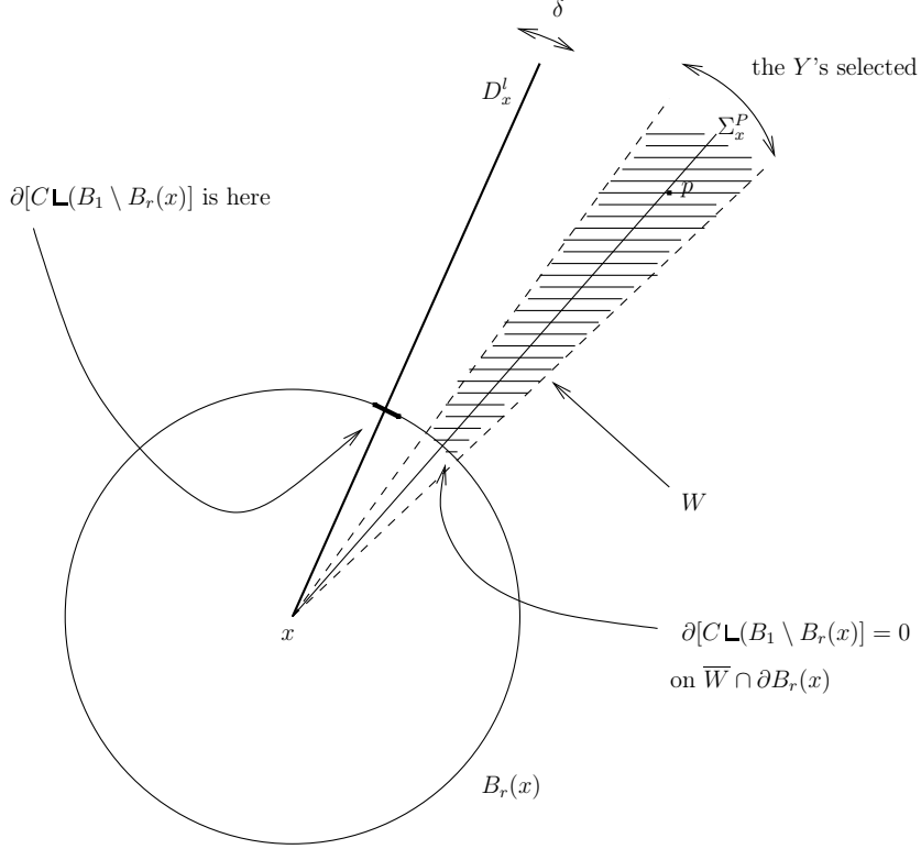
Figure 5: Magnify around x : selection of W (shaded region).
