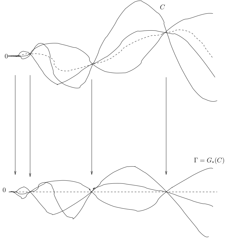
Figure 7: A sketch for a 3-valued graph. The average is the dotted line in the first picture. By subtracting it, we get a new 3-valued graph: the points of multiplicity 3 are turned into zeros. The new 3-valued graph still represents a boundaryless current, thanks to the W^{1,2} -estimate on the average.
