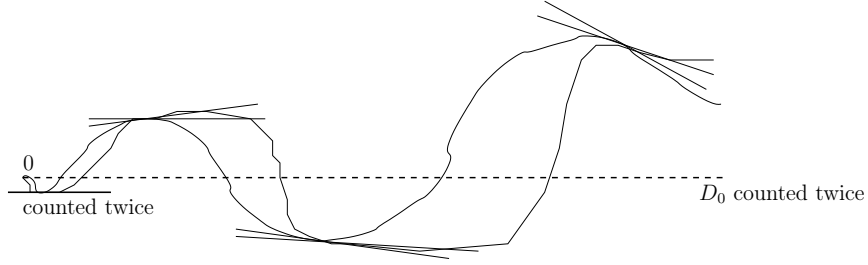
Figure 6: An example for Q = 2 , with the current sketched as two curves. The tangents at points of multiplicity 2 flatten as they approach 0.
