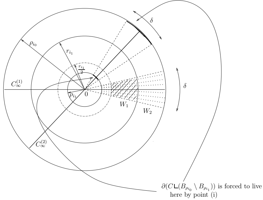
Figure 2: In the picture we have taken C_\infty^{(1)} to be Q times D_0 . C_\infty^{(2)} is a different disk counted Q times. The horizontal and vertical directions should be respectively thought of as [1, 0] and [0, 1] . The fifth direction should be imagined as entering the picture. The dotted region corresponds to W_2 ; its subset W_1 is shaded.
