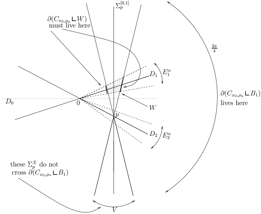
Figure 3: Situation inside the ball B_1 . To avoid confusion in the picture, we imagine that y_n coincides with p . The dotted region corresponds to W . Heuristic idea of the proof: any \Sigma_p^X , X \in V , should intersect C_{x_0, \rho_n} with multiplicity Q near p , since there we have a point of multiplicity Q . But there is mass of C_{x_0, \rho_n} in W and this portion must also give a strictly positive contribution to the intersection index of C_{x_0, \rho_n} and \Sigma_p^X . But now there is too much intersection.
