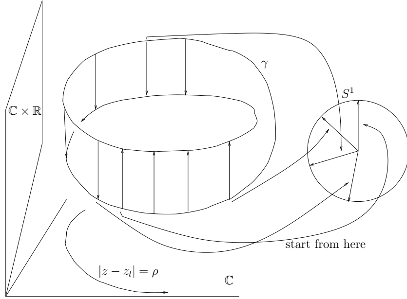
Figure 8: On the left, an attempt to represent \gamma = \pi^{-1}\{|z - z_l| = \rho\} in the case of a two-valued graph in \mathbb{C} \times \mathbb{C} \times \mathbb{R} . We observe the evolution of the difference vector joining points above the same z \in \{|z - z_l| = \rho\} \subset \mathbb{C} : as the tail of the difference vector runs along \gamma , we keep track (picture on the right) of the normalized difference vector projected on the second \mathbb{C} -factor and observe how it winds around S^1 . If we are around an isolated singularity, then we find that the represented map from \gamma to S^1 has strictly positive degree. In this particular picture, after having run once along \gamma the normalized difference vector winds once positively around S^1 .
