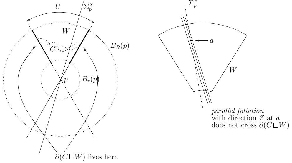
Figure 1: On the left: schematical view of the statement. C is dashed. Due to the condition on the boundary of C \llcorner W , for any \Sigma_p^X with X \in U we must find a strictly positive intersection index. On the right: the choice of the parallel foliation near a .
