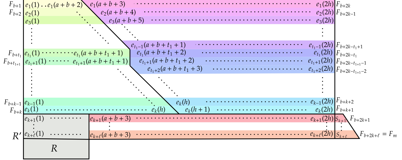
Figure 1: An illustration of how the graph G is partitioned into (F_{b+1}, \dots, F_m, R') . Here all the edges of G are pictured in the way we get them from Lemma 22 at the start of the proof — either as edges e_i(j) of H_i , the stars S_i , or the remainder R . The isomorphic graphs H_i are arranged in a rectangle so that any subset of edges e_i(j) in row i is isomorphic to the corresponding subset on any other row. The coloured areas represent the final partition (F_b, \dots, F_m, R') which ends up satisfying the lemma.
