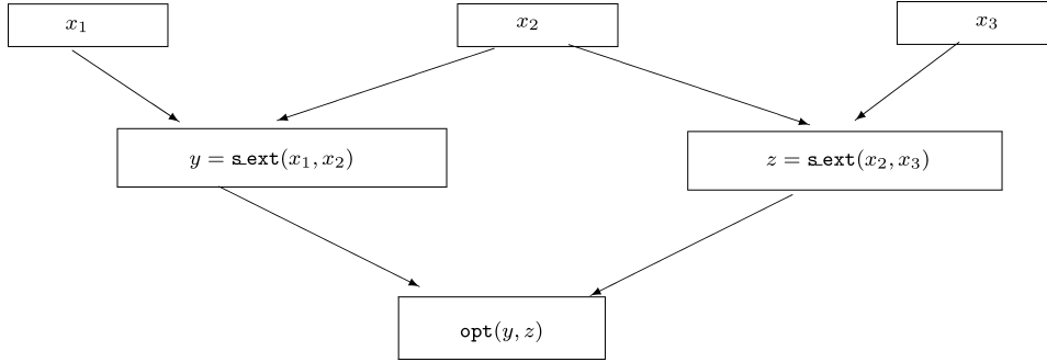
FIG. 6. A 3-source extractor.
