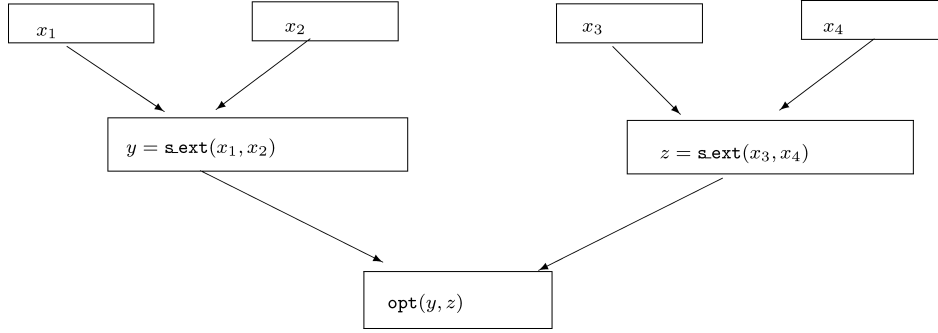
FIG. 5. A 4-source extractor.
