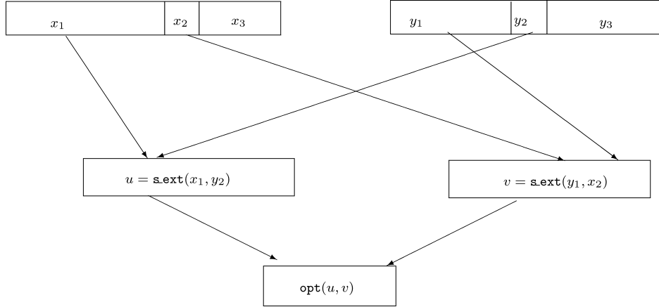
FIG. 9. The output \text{disp}_I(x, y) with respect to partition I .
