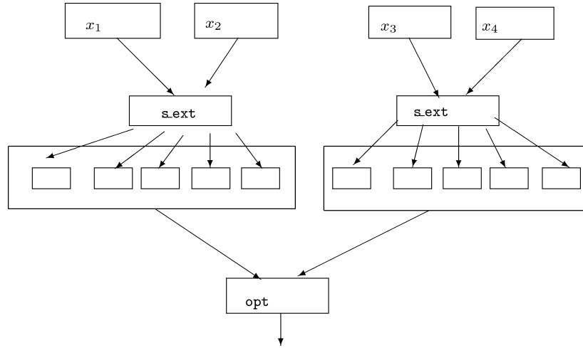
FIG. 2. A 4-source extractor 4\text{ext} .
