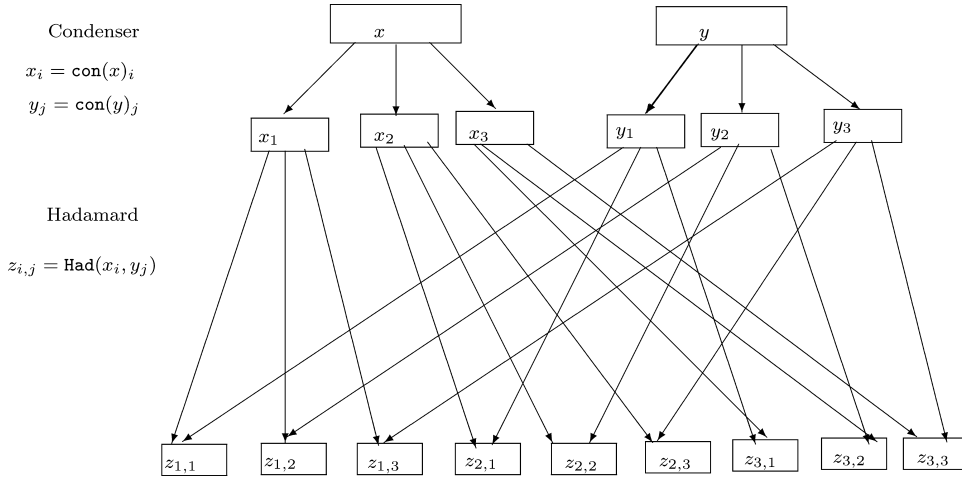
FIG. 4. A (2-source) Somewhere-Extractor.
