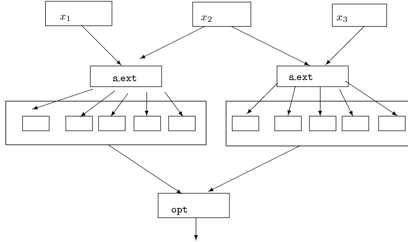
FIG. 3. A 3-source extractor \mathfrak{3ext} .
