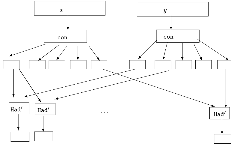
FIG. 1. A 2-source somewhere extractor s\_ext .
