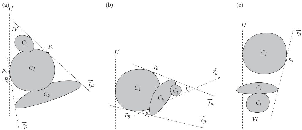
FIGURE 6. Regions IV, V, and VI. (a) In Region IV, (C_j, C_k, C_l) has a strong counterclockwise orientation. (b) In Region V, C_l \subset \text{conv}(C_j \cup C_k) . (c) In Region VI, (C_i, C_j, C_l) has only a strong clockwise orientation.
