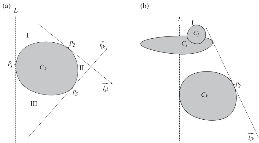
FIGURE 3. Regions I, II, and III. (a) C_l \setminus C_k must lie in either Region I, II, or III. (b) (C_j, C_k, C_l) does not have a strong clockwise orientation.
