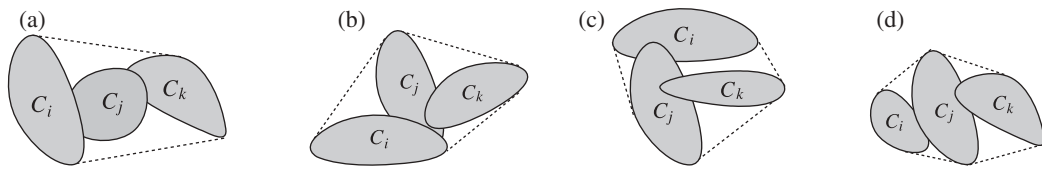
FIGURE 1. Orientations of convex bodies. (a) (C_i, C_j, C_k) not in general position. (b) Clockwise orientation. (c) Counterclockwise orientation. (d) Both orientations.
