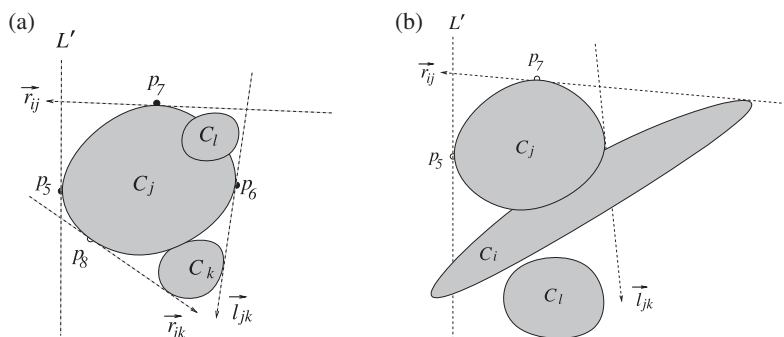
FIGURE 8. Regions VII and VIII. (a) In Region VII, (C_j, C_k, C_l) has a strong counterclockwise orientation. (b) In Region VIII, (C_i, C_j, C_l) has only a strong clockwise orientation.
