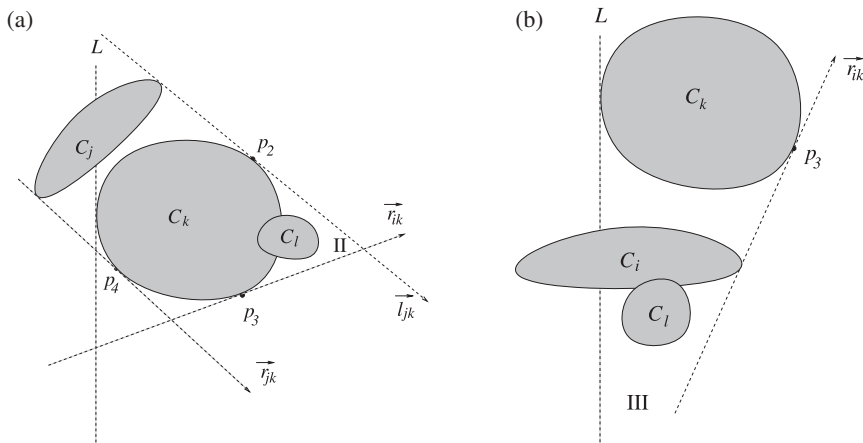
FIGURE 4. Regions II and III. (a) C_l \setminus C_k lies in Region II implies (C_j, C_k, C_l) has both strong orientations. (b) (C_i, C_k, C_l) has only a strong clockwise orientation.
