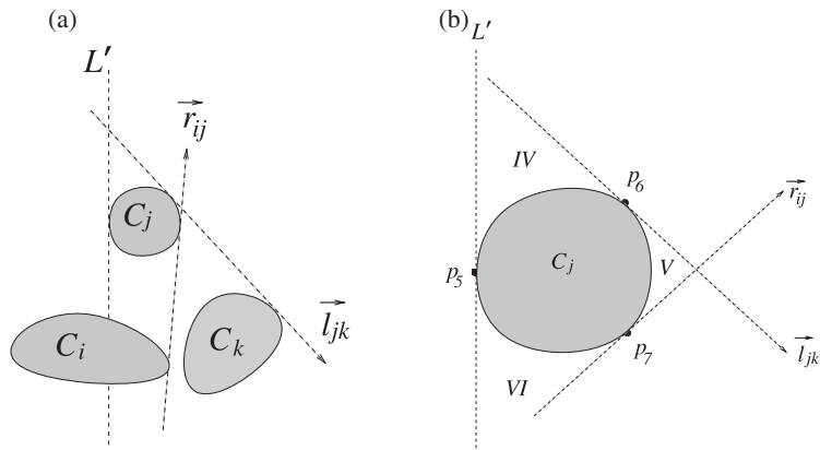
FIGURE 5. Regions IV, V, and VI. (a) (C_j, C_k, C_i) separable. (b) Regions IV, V, and VI.
