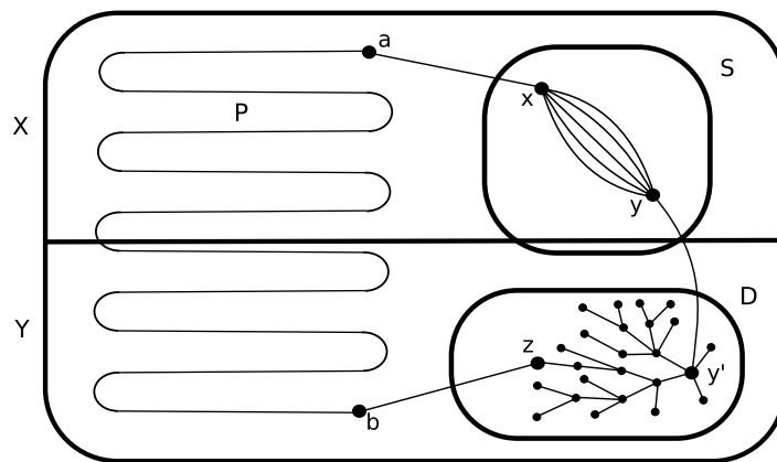
Fig. 1. Constructing cycles of intermediate length.
