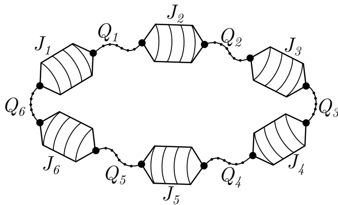
FIG. 3. A gadget-cycle.
