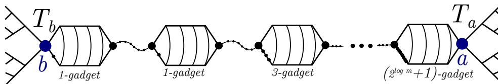
FIG. 2. Constructing a (\leq 2^{\lceil \log m \rceil}) -gadget in the proof of Lemma 2.15.
