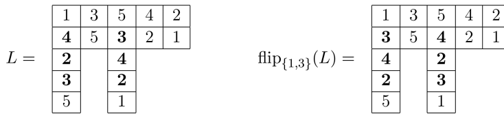
FIGURE 2 We show the effect of the flip operation. Note that \sigma_{1,2}(L) = (145)(23) and \sigma_{1,2}(\text{flip}_{\{1,3\}}(L)) = (12345)
