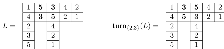
FIGURE 1 We show the effect of the turn operation. (Not all cells are depicted). Note that \{1, 3\} was not flippable in L but is flippable in \text{turn}_{\{2,3\}}(L) . Also note that \sigma_{1,2}(L) = \sigma_{1,2}(\text{turn}_{\{2,3\}}(L)) = (1\ 4\ 5)(2\ 3)
